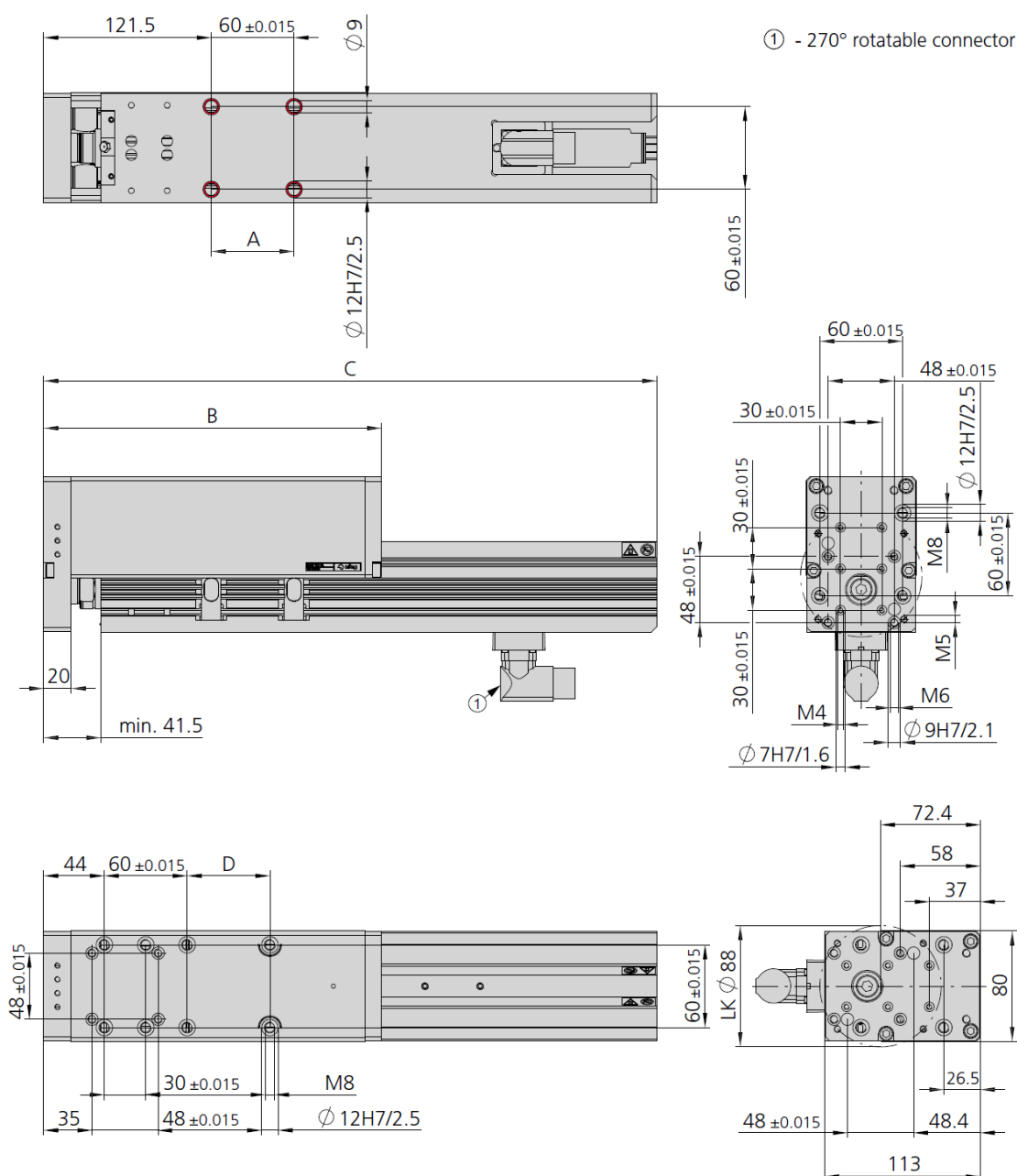
Fig. 1 Dimensional drawing of electric slide ES40
