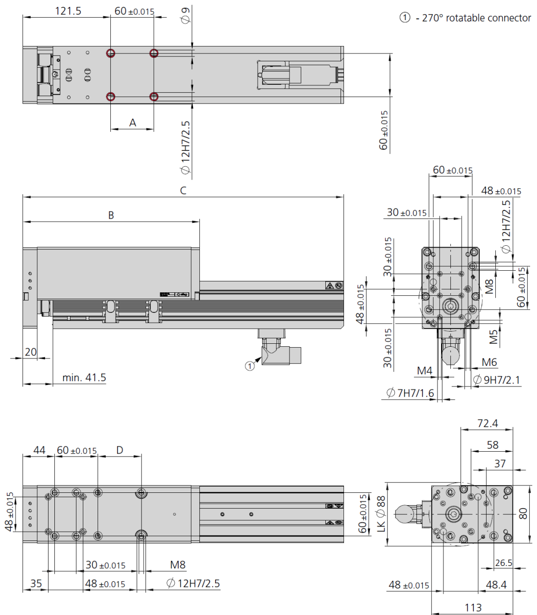
Fig. 2 Dimensional drawing of electric slide ES40-HP
