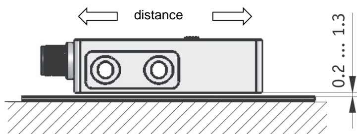
Fig. 9 External position measuring system (example illustration)
