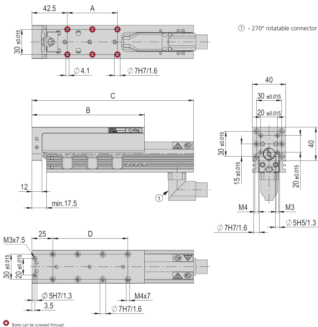
Fig. 1 Dimensional drawing of electric slide ES20
