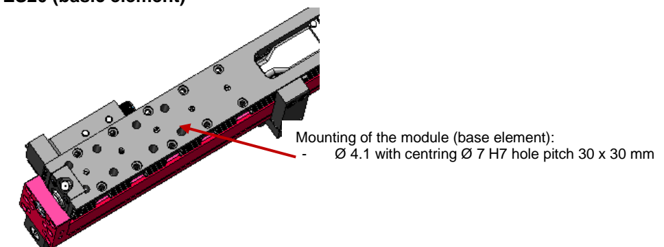
Fig. 14 Electric slide ES 20 (mounting basic element)
