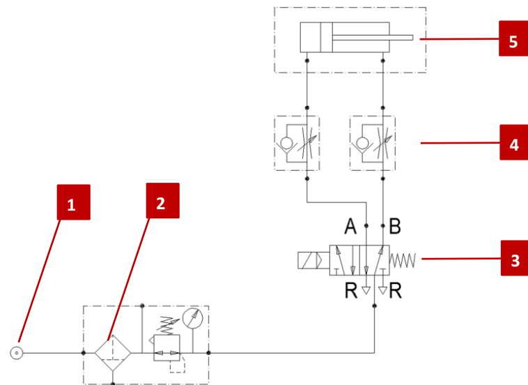
Abb. 12 Pneumatik-Schaltplan Compact-Schlitten (5/2)
