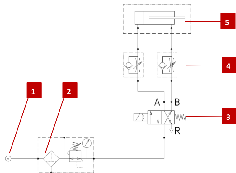
Abb. 13 Pneumatik-Schaltplan Compact-Schlitten (4/2)
