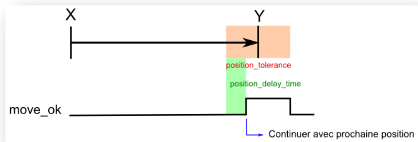
Figure 19: Mode Position
