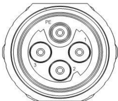
Figure 4: Vue des branchements [X1]
