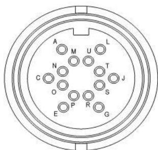
Figure 15: Vue des branchements [X6]
