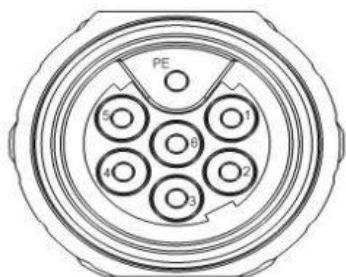
Figure 14: Vue des branchements [X5]
