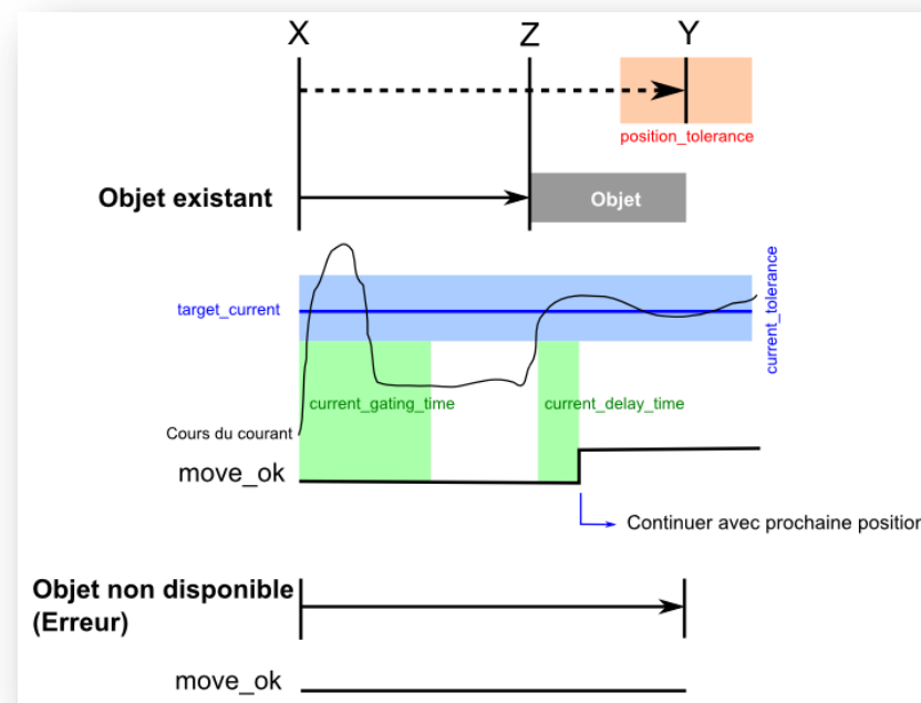
Figure 20: Mode Courant
