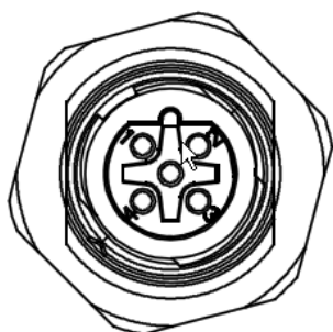
Figure 7: Vue des branchements [X3b]
