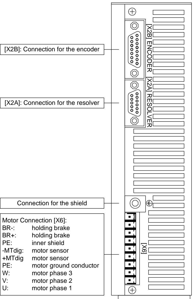
Figure 3: Servo positioning controller SE-POWER: Bottom view
