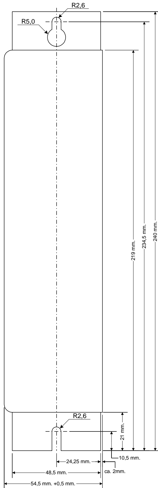
Figure 5: Servo positioning controller SE-POWER: Mounting plate Electrical installation
